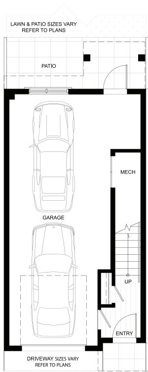
FIRST FLOOR
